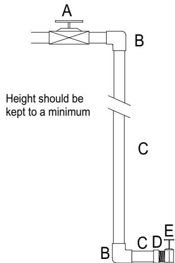
Sludge Line
